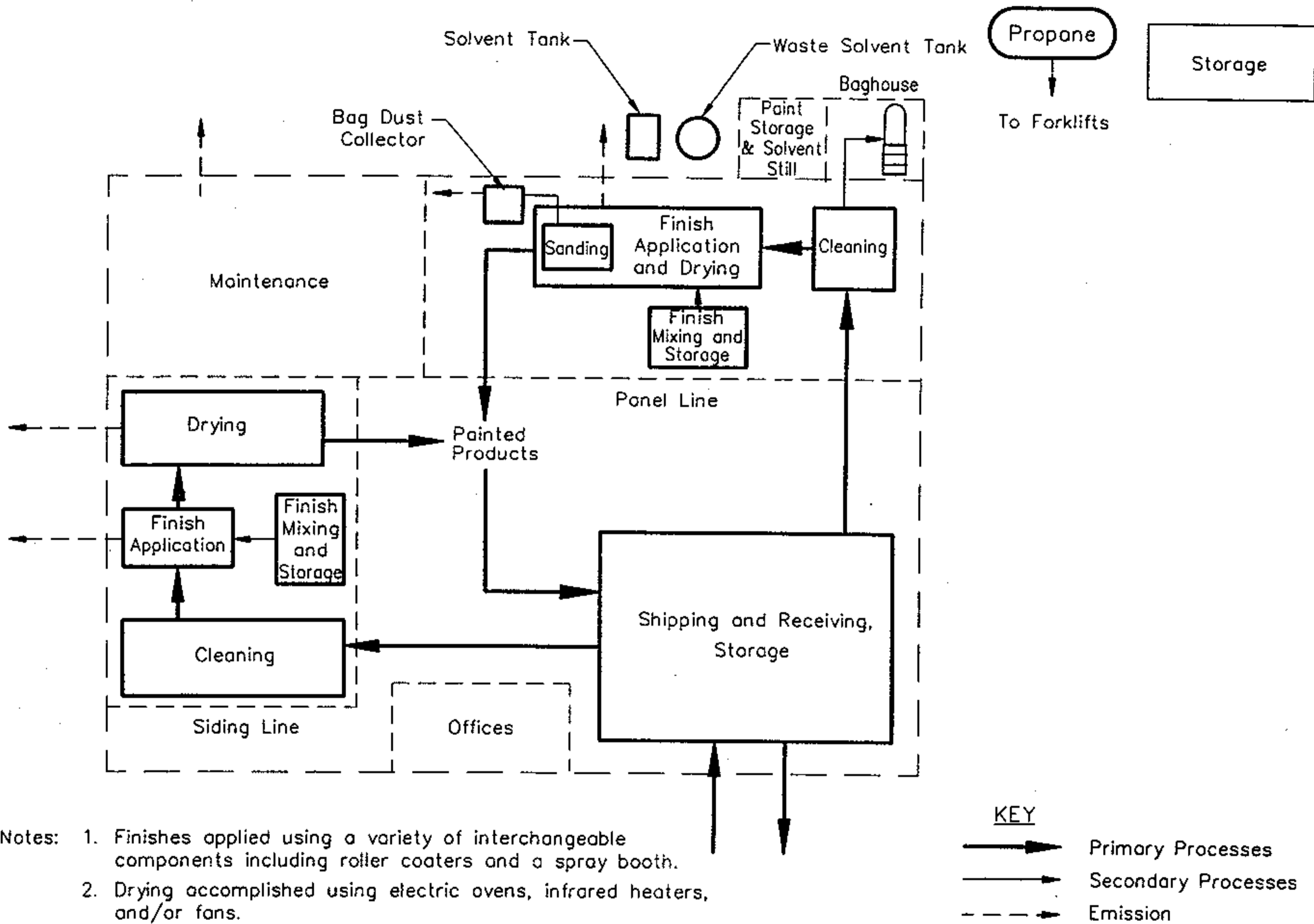
Girard Custom Coaters Process Flow Diagram
